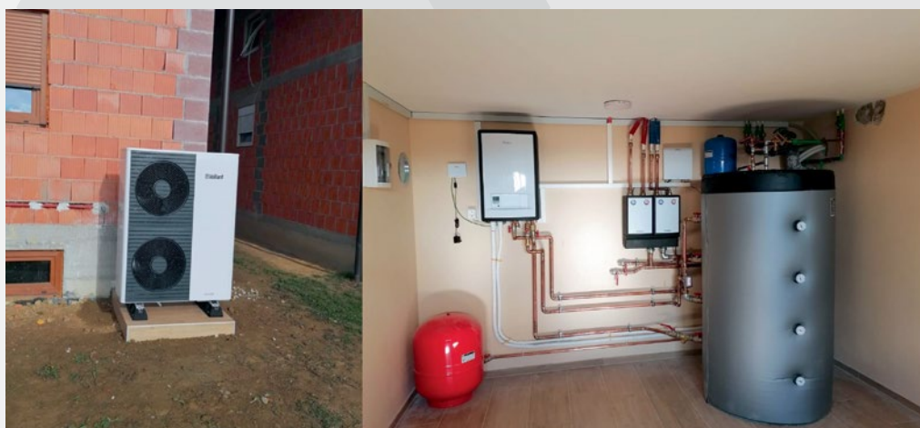
Dizalica topline aroTHERM VWL 125 u Sibinju
